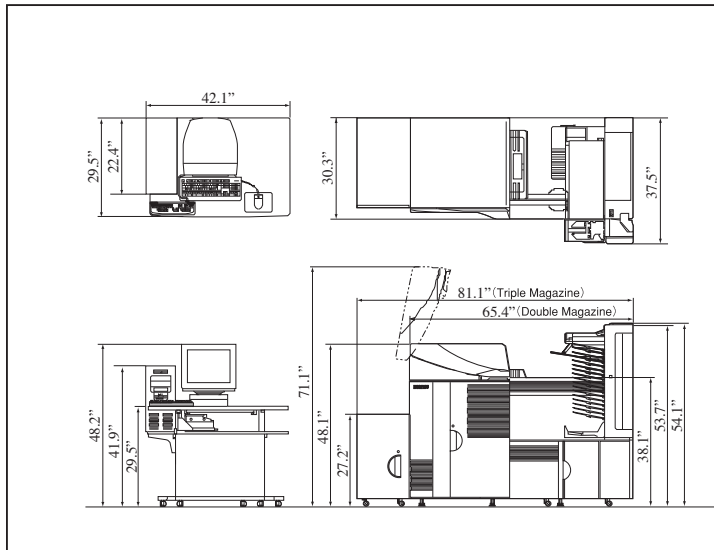
QSS-3202/3203 PRO External view
