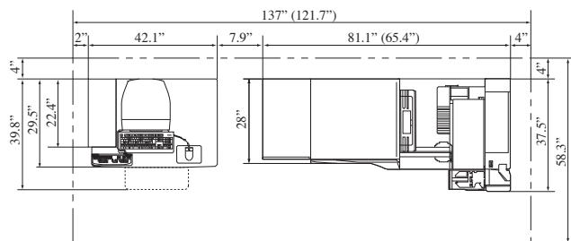
QSS-3202/3203 PRO Space required for installation
